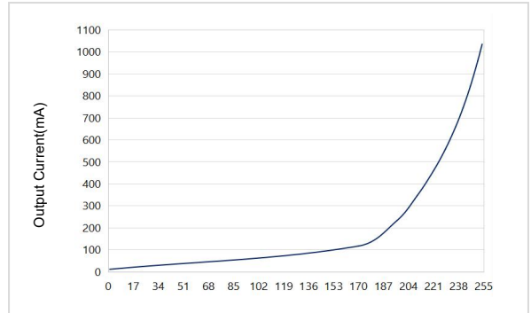
logarithmic dimming
